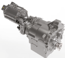
e-Powershift Transmission
